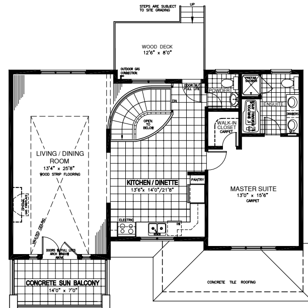
SECOND FLOOR PLAN 1045 sq.ft.
