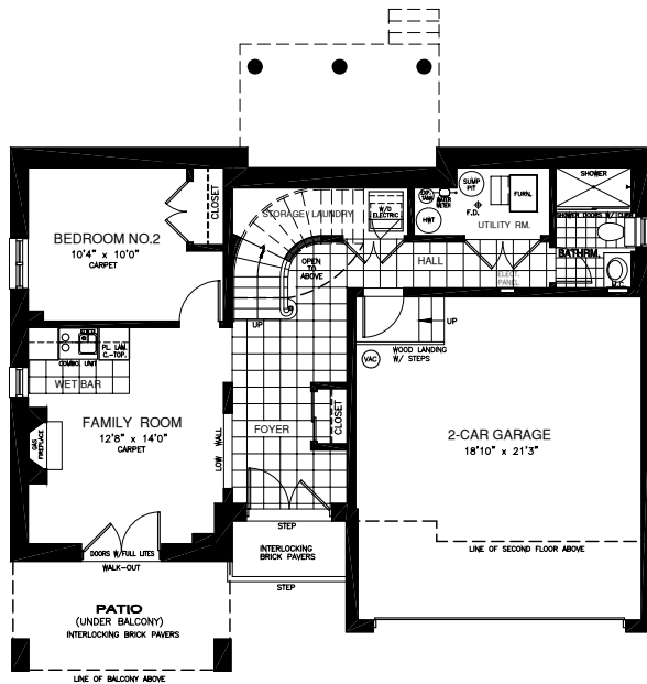
GROUND FLOOR PLAN 755 sq.ft.
